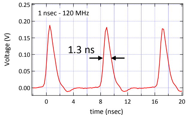
Time Profile of Pulse Output
