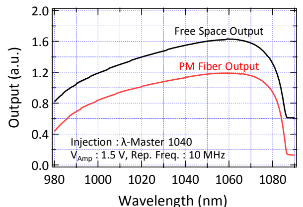
Injection Wavelength Dependence
